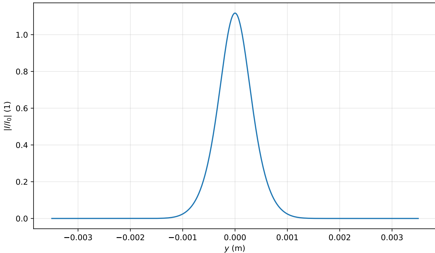
Intensity profile I(x=0, y, z=0.876)/I_0 , P_{in}=0.6P_{cr} , artificial time
